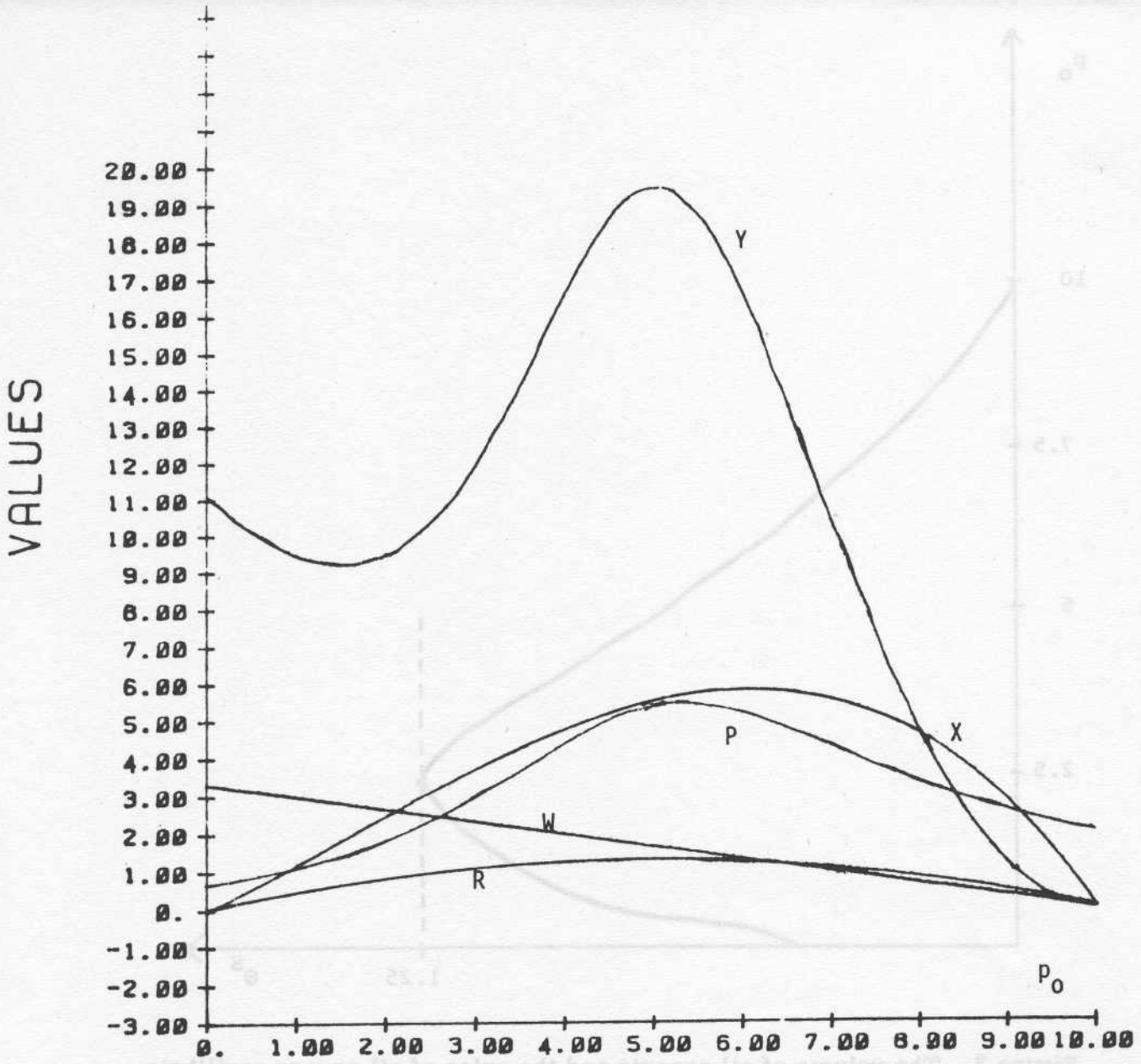
Figure 4. Results from a simulation: note that the GDP, Y, of the oil importer rises and then falls with increases in the price of oil, p_0 .
